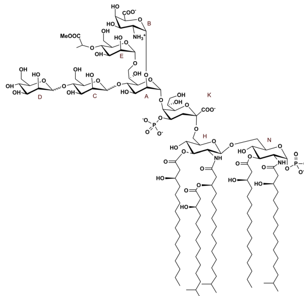
Fig. 4 Full structure of the LOS from O. splanchnicus . Branched fatty acids are represented in their iso-form; however they can also be found as linear or anteiso chains.
