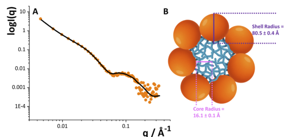
Fig. 5 (A) SAXS experimental data and best fit for the O. splanchnicus LOS in water. (B) Schematic depiction of the spherical micelle, showing the hydrophobic lipid A core (light blue) enveloped by the oligosaccharide shell (orange).
